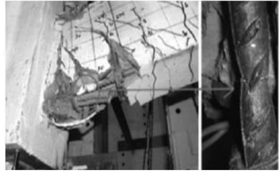
Figure (12) Experimental Crack Pattern [18].
