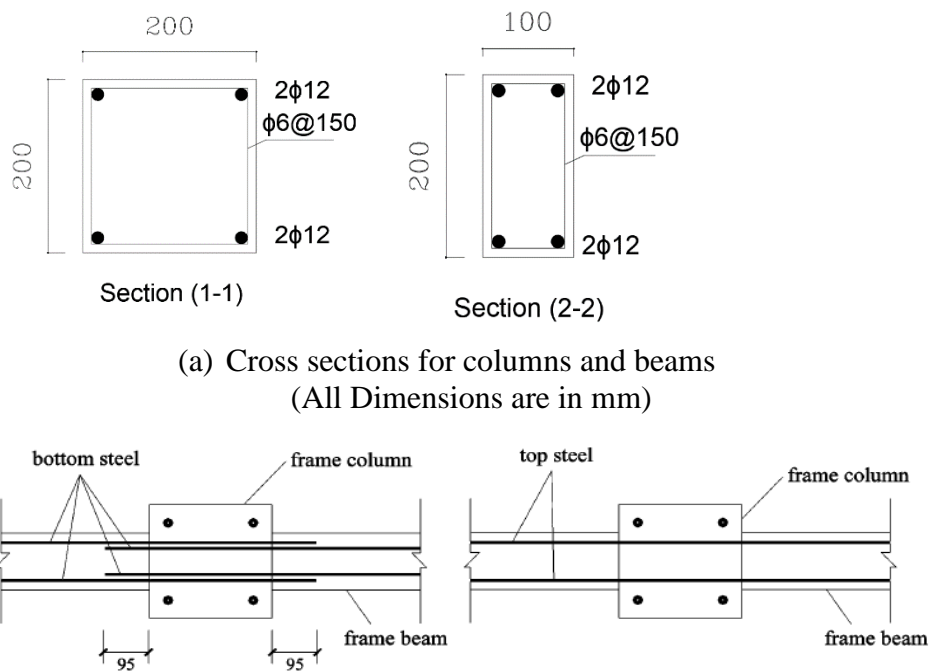
(b) Plan of the top and the bottom beams reinforcement bars extensions
