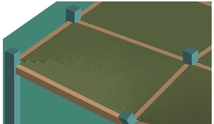
Figure (31) Experimental and Numerical Cracks at the Longitudinal Beam for the 3-D Single-Story Frame [21].
