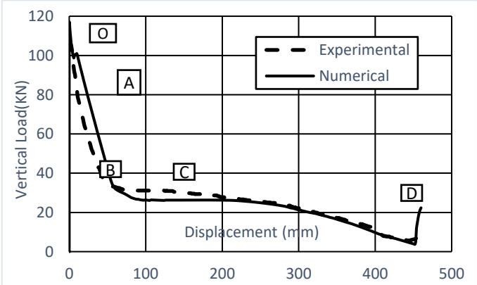
Figure (14) Experimental vs. Numerical Load-Displacement Curve.
