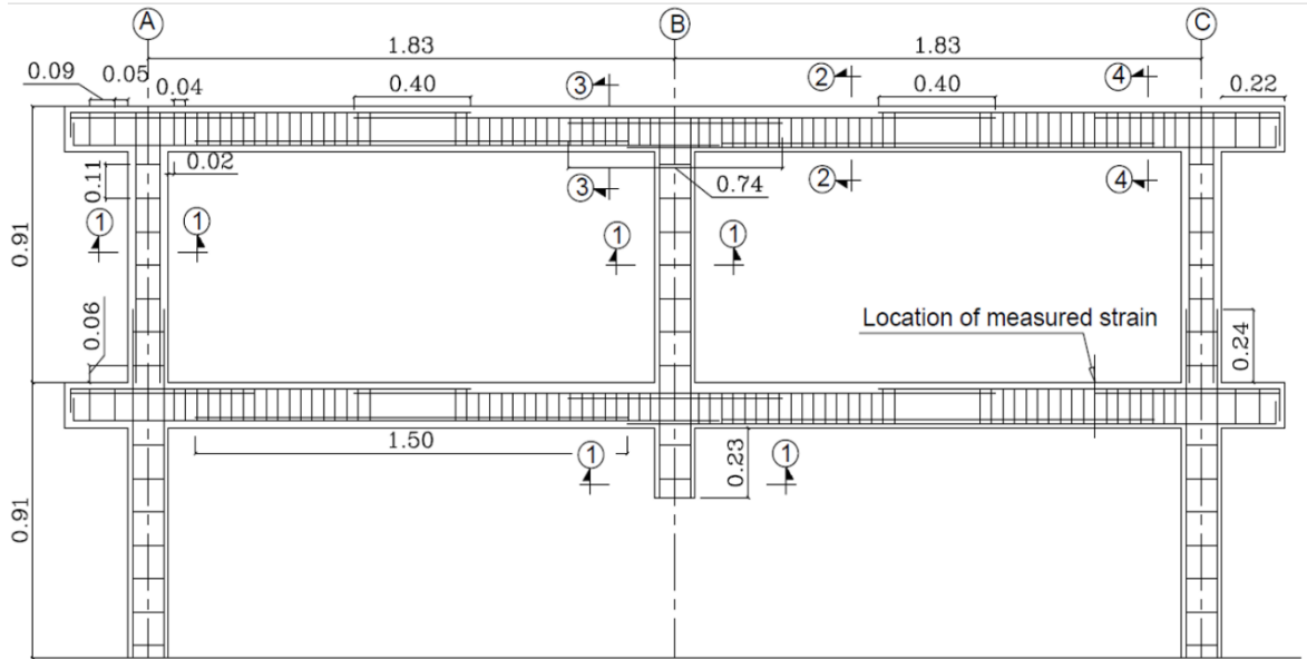
Figure (16) Concrete Dimensions and Reinforcement Details of 2-D 2-Story Frame [19] (All Dimensions are in mm).
