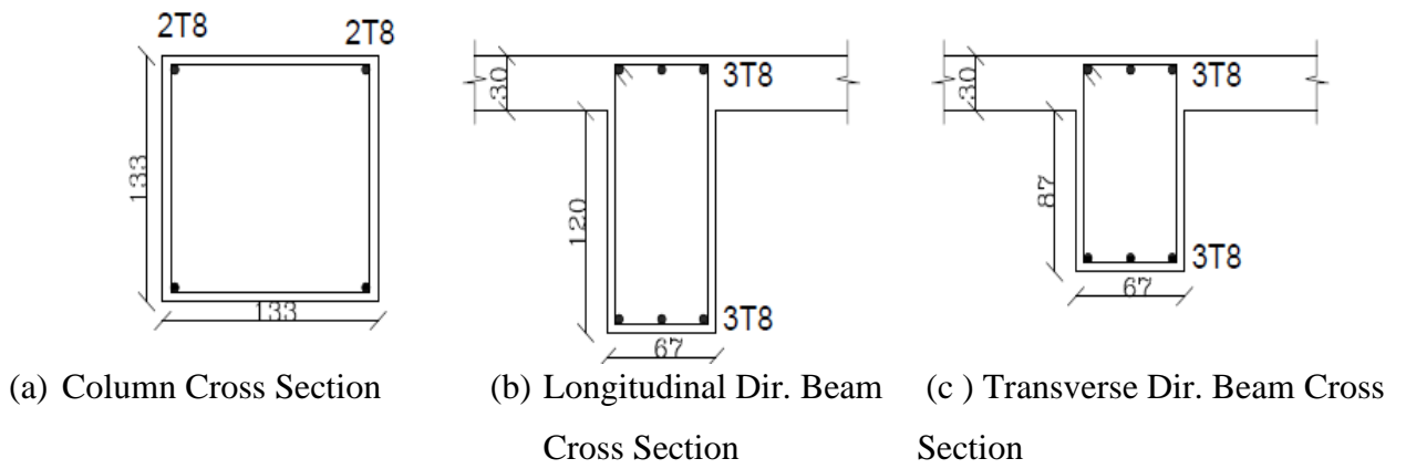
Figure (23) Beams and Columns Cross-Sections for the 3-D Single-Story Frame [20].
