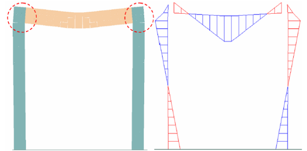
Figure (5) Case 2: Reinforcement of Beam is Extended in the Column (Rigid Connection).
