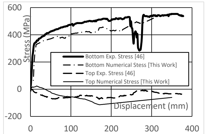
Figure (35) Experimental vs. Numerical Steel Stress at Position (2) for the 3-D Single-Story Frame [21].
