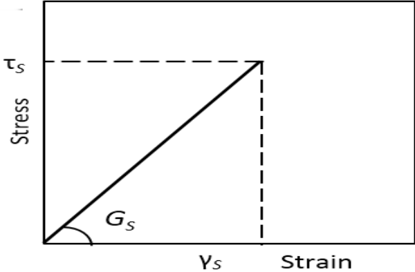
Figure (9) Shear Model for reinforcing Steel [17].
