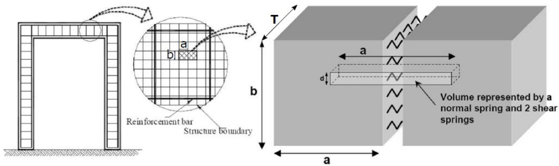
Figure (2) Modelling of Structure using AEM [11].
