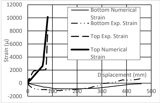
Figure (15) Experimental vs. Numerical Steel Strain Curve.
