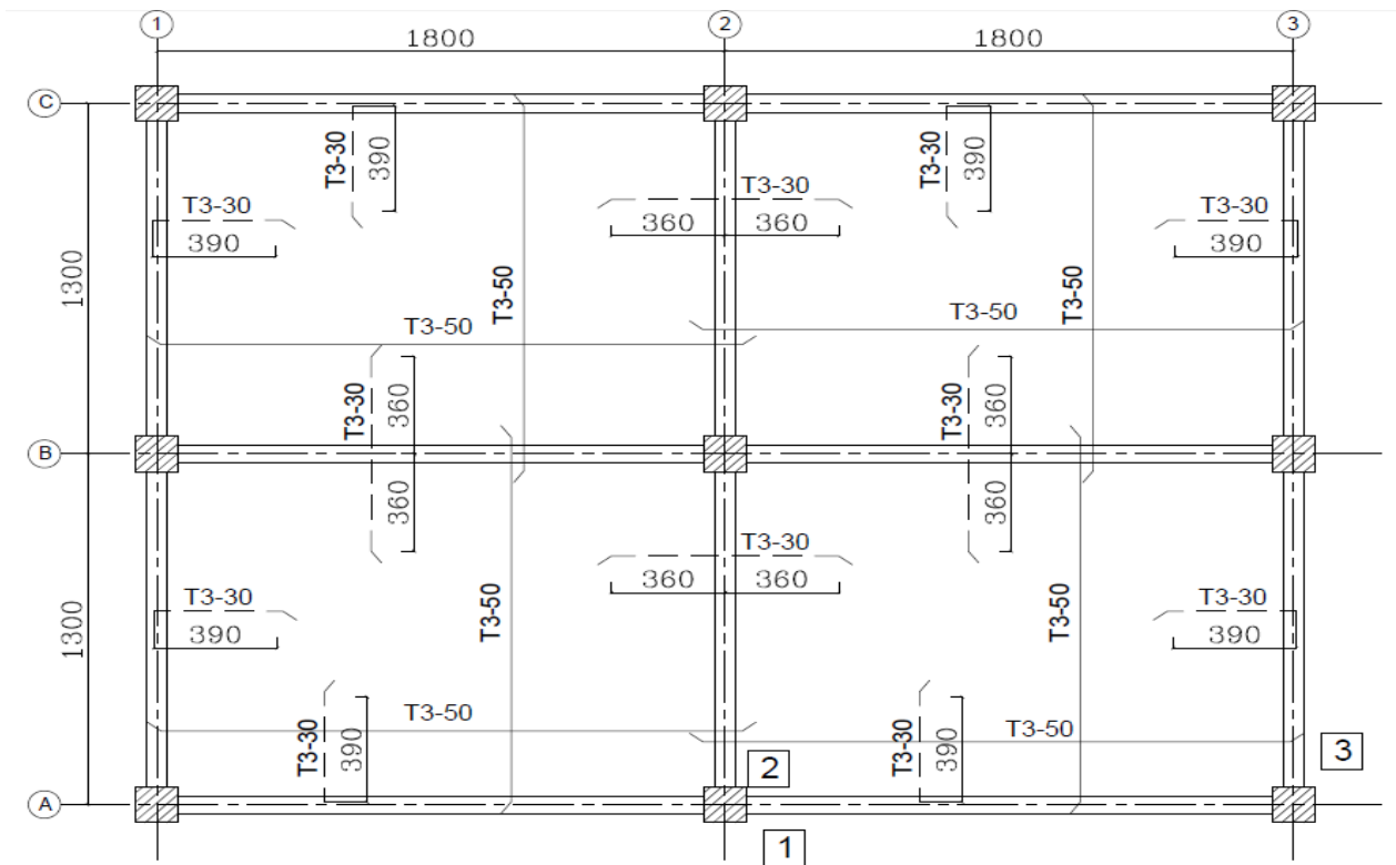
Figure (29) Layout of the Slabs and its Reinforcement Arrangement for the 3-D Single-Story Frame [21] (All Dimensions are in mm).
