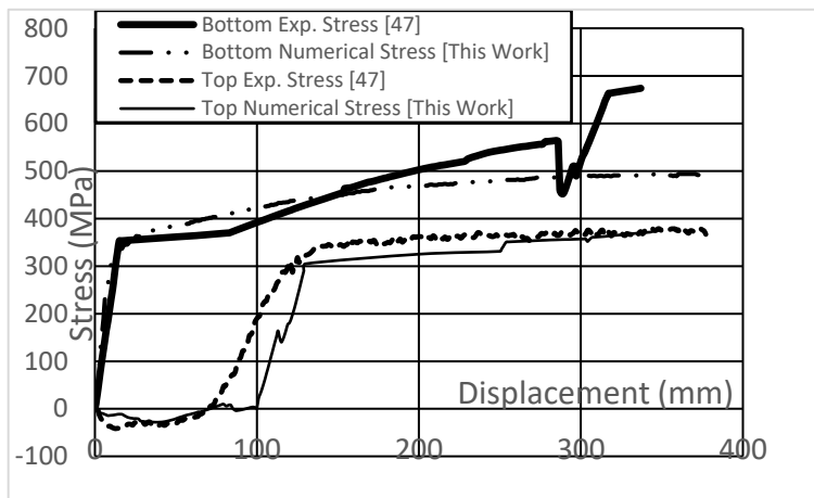
Figure (34) Experimental vs. Numerical Steel Stress at Position (1) for the 3-D Single-Story Frame [21].
